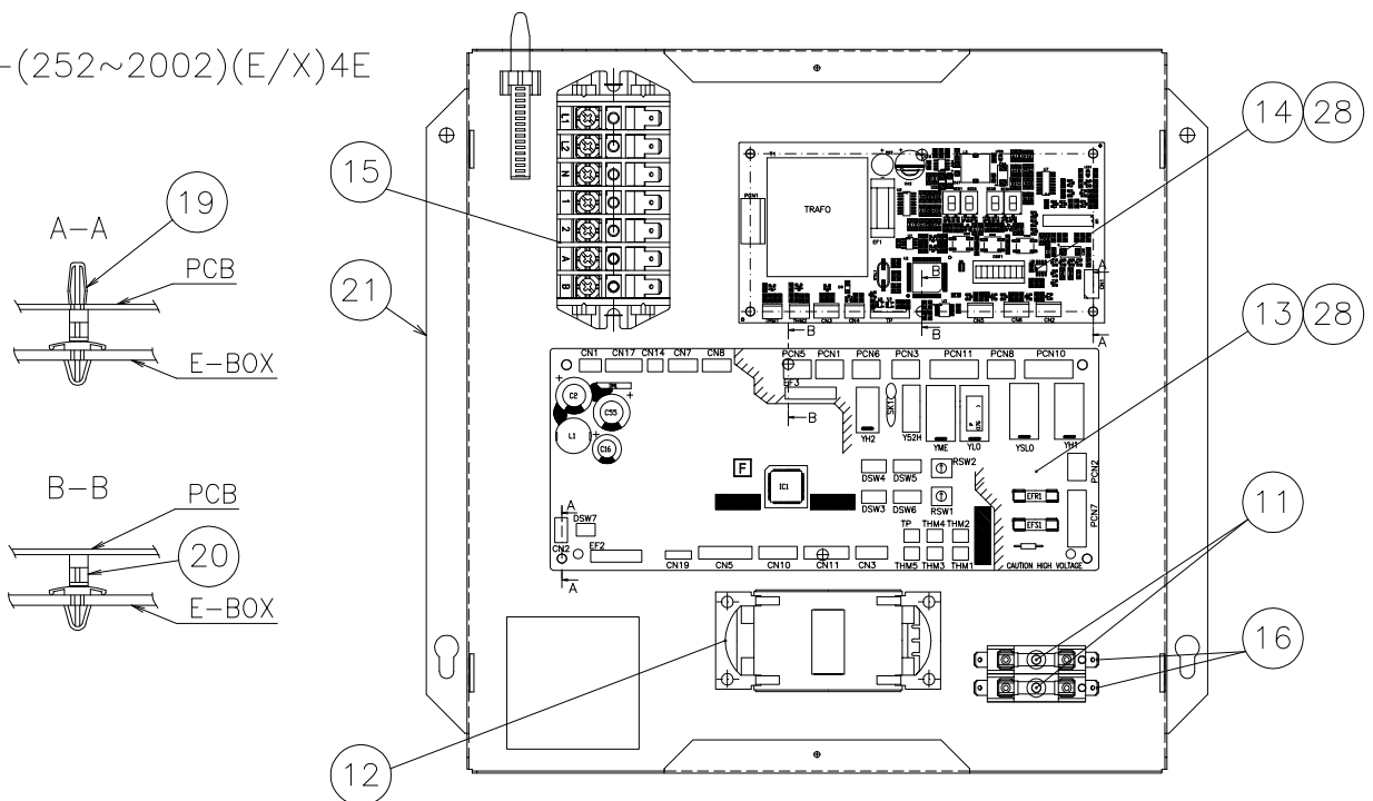
LOCATION OF ELECTRICAL EQUIPMENT IN THE ELECTRICAL BO
